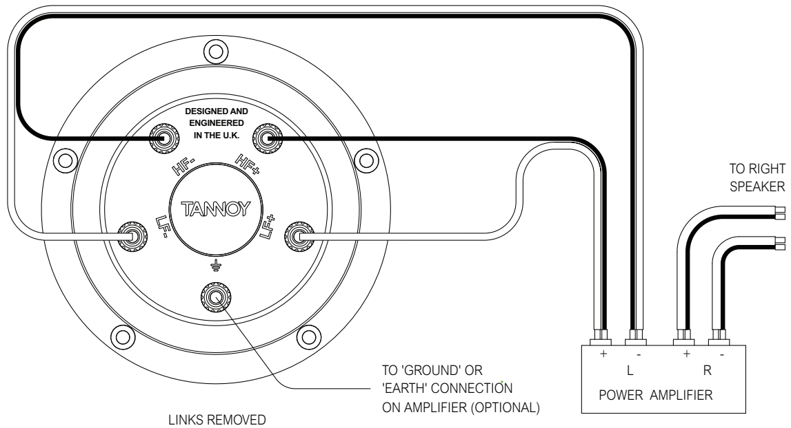
Fig.5 Bi-Wire Mode
