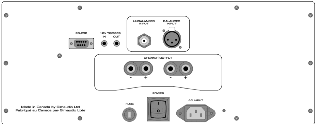
Figure 1: Rear panel of Moon W-7M Mono Amplifier
