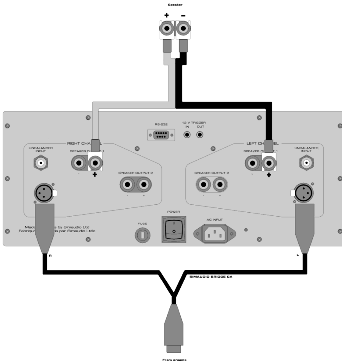
Figure 3: Bridged-Mono operation of the MOON 870A Dual-Mono Amplifier
