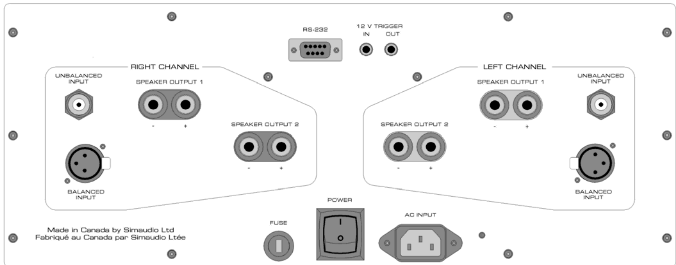
Figure 1: Rear panel of Moon 870A Dual-Mono Amplifier
