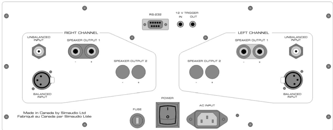
Figure 1: Rear panel of Moon 860A Dual-Mono Amplifier
