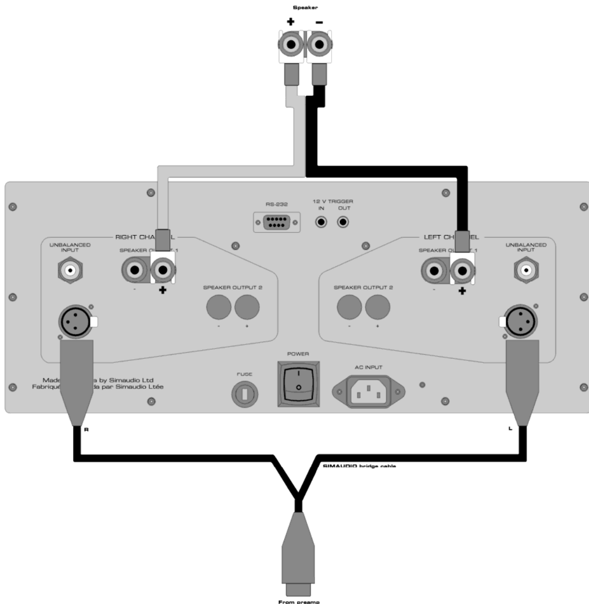
Figure 3: Bridged-Mono operation of the MOON 860A Dual-Mono Amplifier
