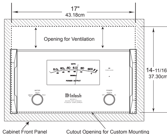
MC601 Front Panel Custom Cabinet Cutout
