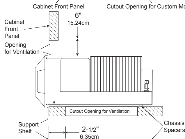
MC452 Side View in Custom Cabinet
