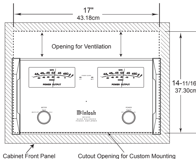
MC452 Front Panel Custom Cabinet Cutout
