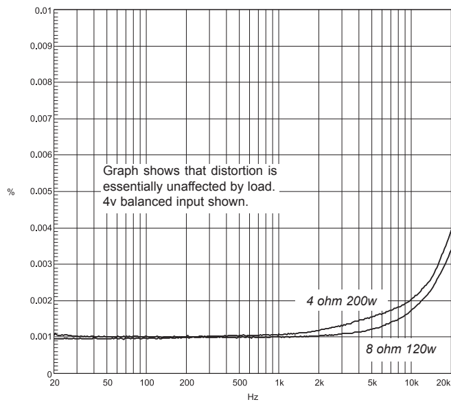
Typical THD+N Sweep
