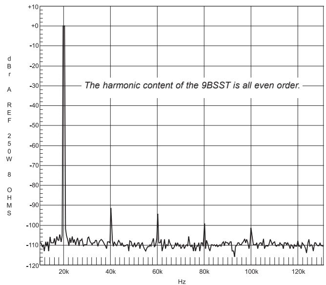
Typical THD+N Harmonic Content
