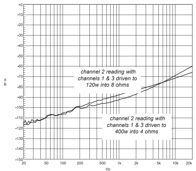
Typical Crosstalk
