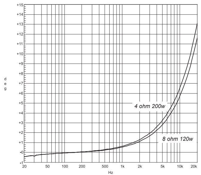
Typical Phase Response
