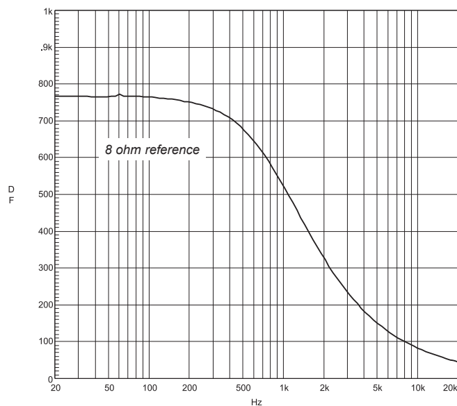
Damping Factor
