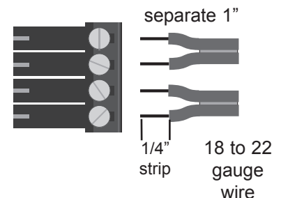
figure W Control voltage wire preparation for screw terminal connector
