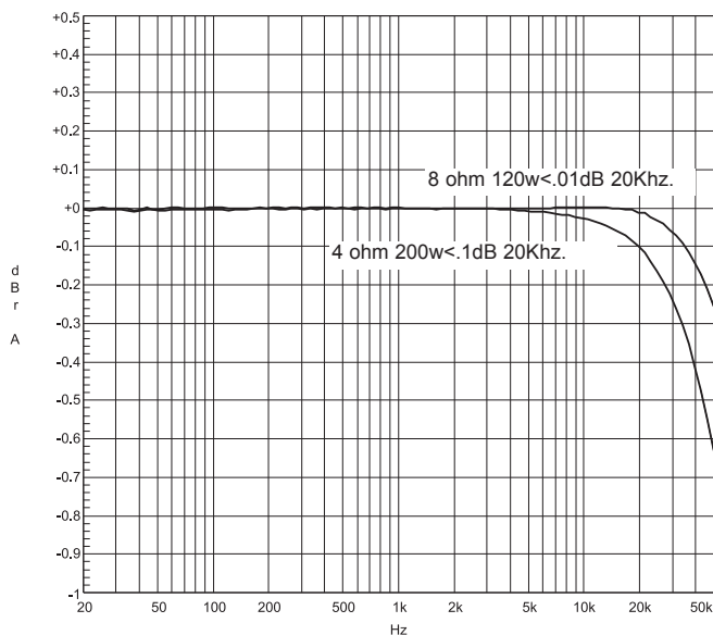
Typical Frequency Response
