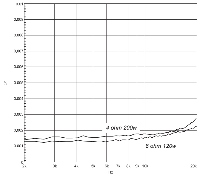
Typical IMD Sweep
