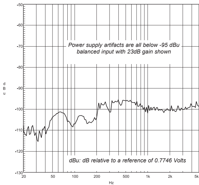
Typical Band-pass Noise
