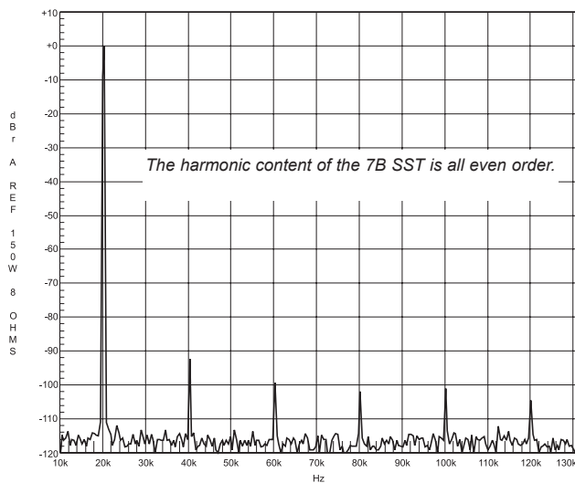
Typical THD+N Harmonic Content
