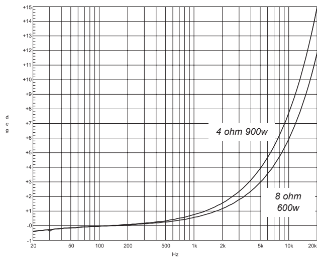
Typical Phase Response
