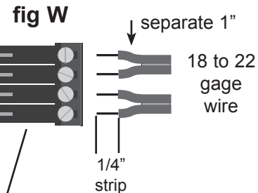
Control voltage wire preparation for screw terminals
