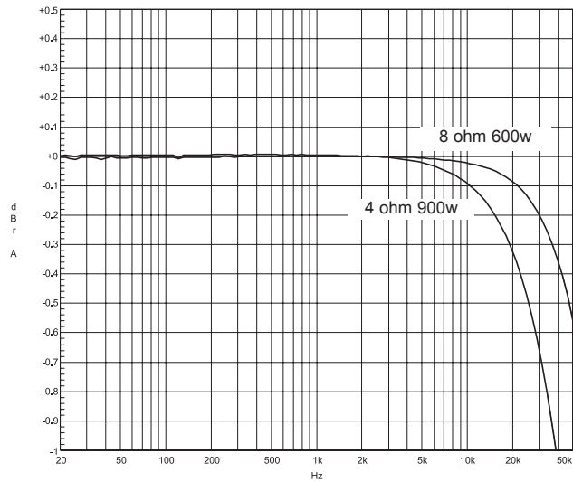
Typical Frequency Response 7BSST
