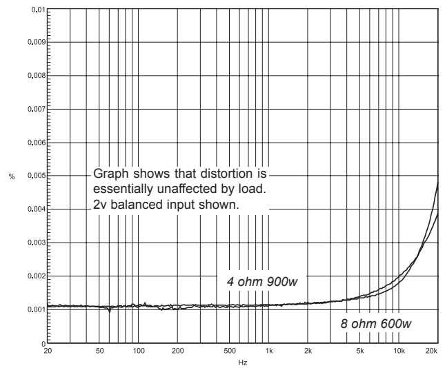
Typical THD+N Sweep
