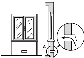
Examples of Ventilation Openings Comburent Air Fig. A
